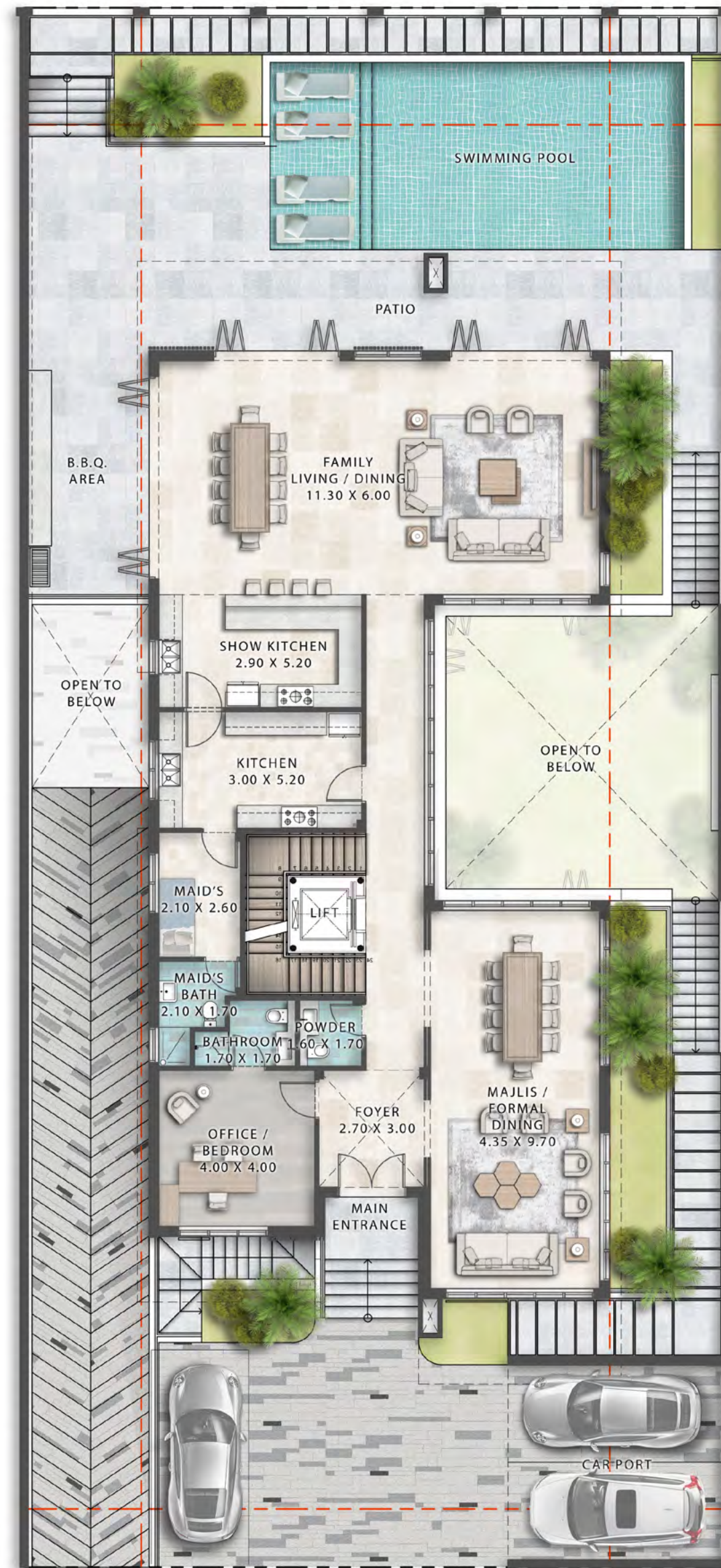
GROUND FLOOR
